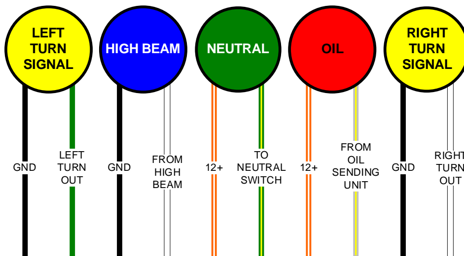
(OEM Colors) Indicator Lights
