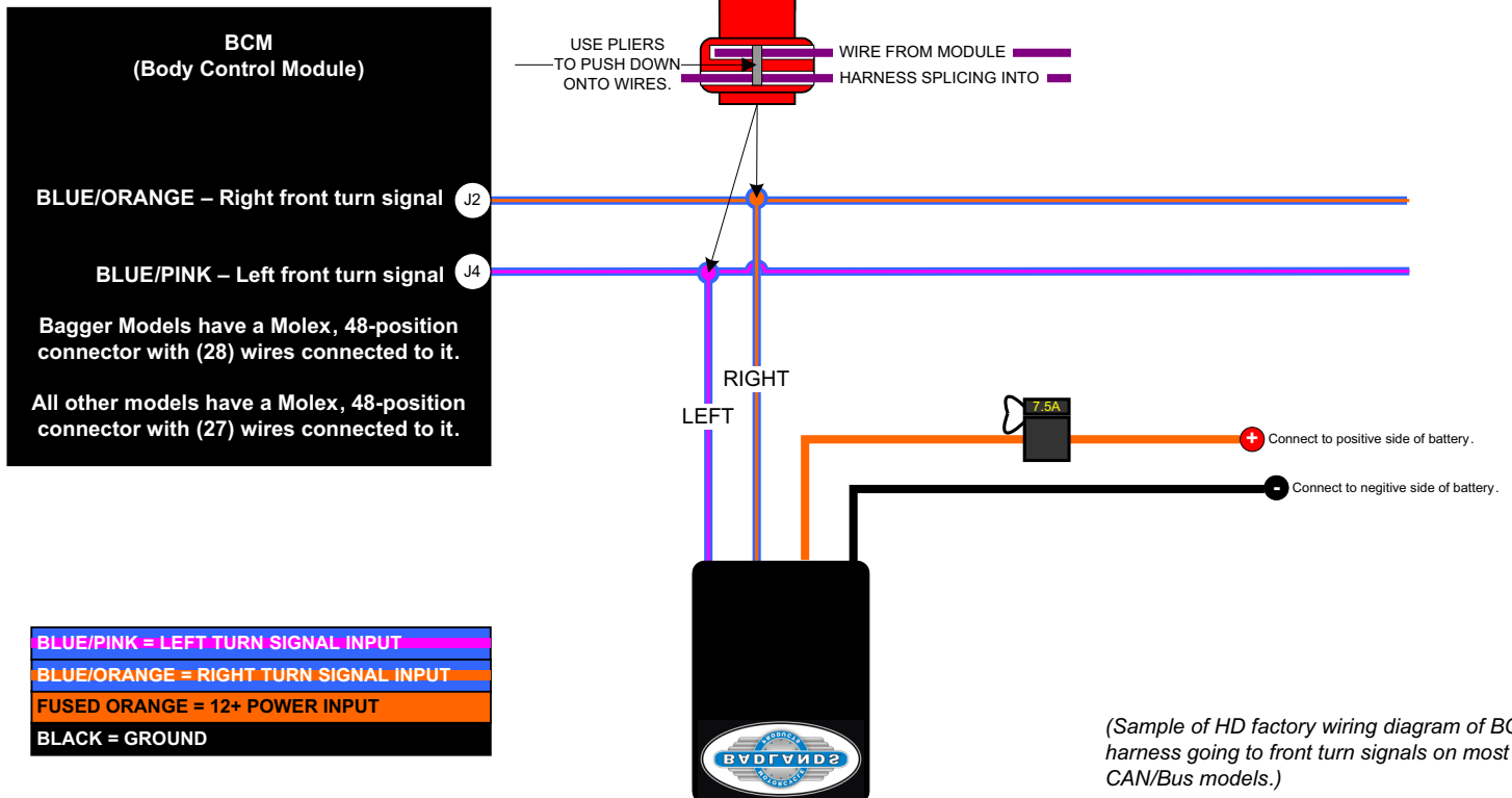
DIAGRAM OF QUICK SPLICE INSTALLATION
